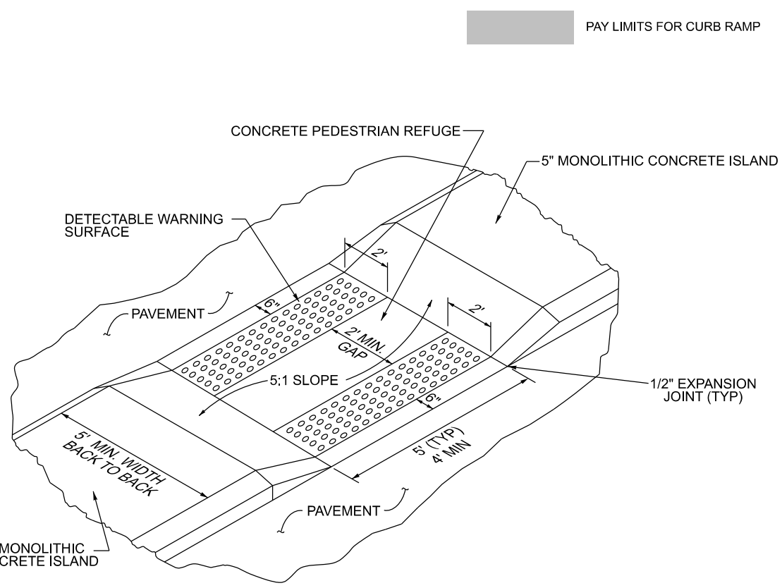
MEDIAN ISLAND WITH CUT THROUGH
